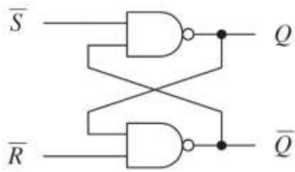
SR-NAND
